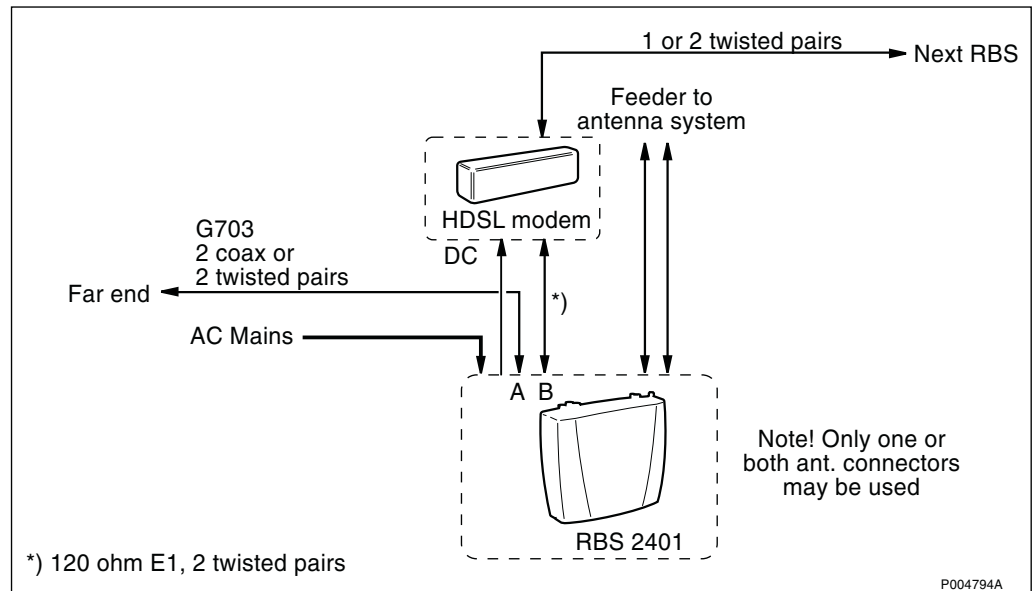
Figure 29 2 TRX with HDSL-modem, G.703/HDSL (R1H1)
