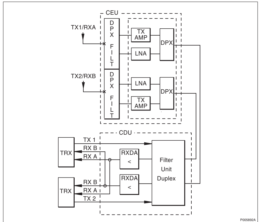
Figure 36 Basic configuration M9d_2.2\C
