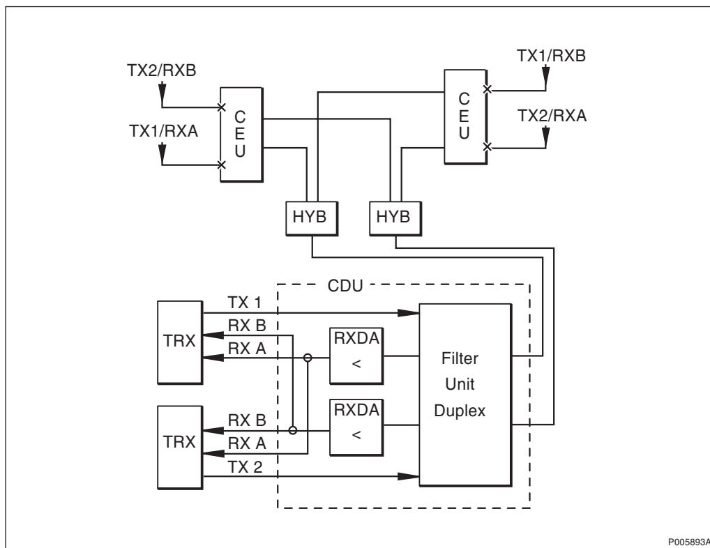
Figure 37 Basic configuration M9d_2.2\H
