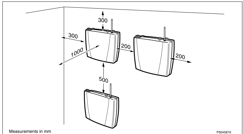
Figure 65 Required space for service
