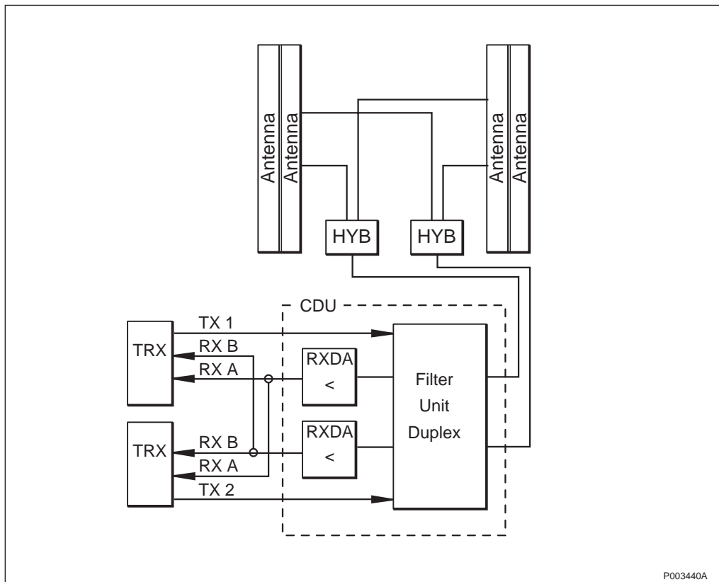
Figure 41 Basic configuration M18d_2.2\H
