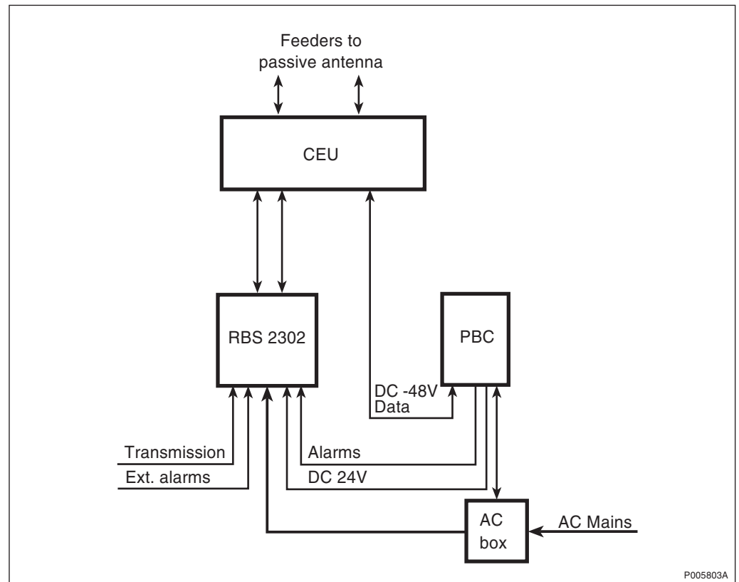
Figure 12 Basic Configuration 2 TRX (R1P1A1)
