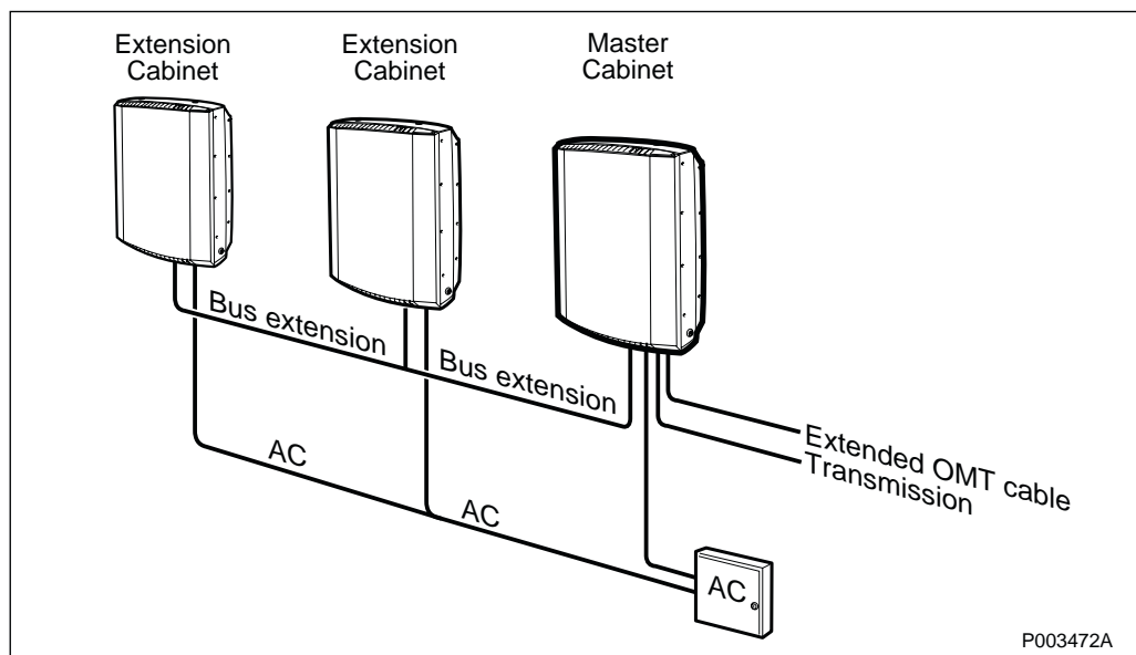
Figure 55 6 TRX site
