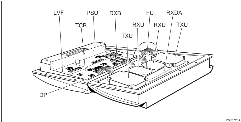
Figure 50 Hardware units in cabinet
