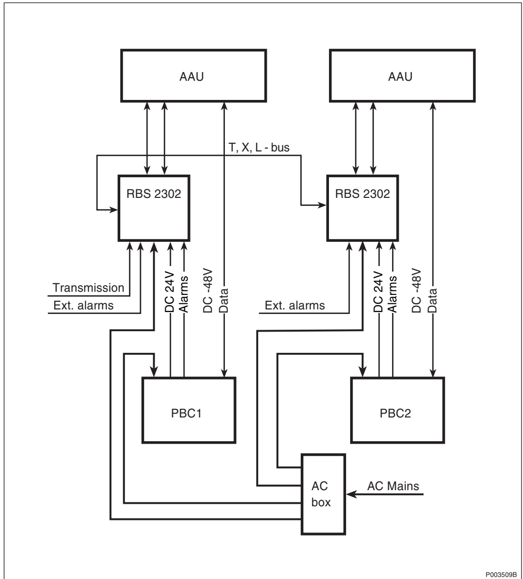
Figure 17 Basic configuration 4 TRX (R2P2A2)
