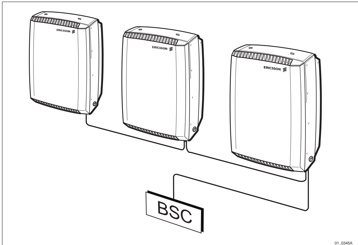
Figure 60 Multidrop chain
