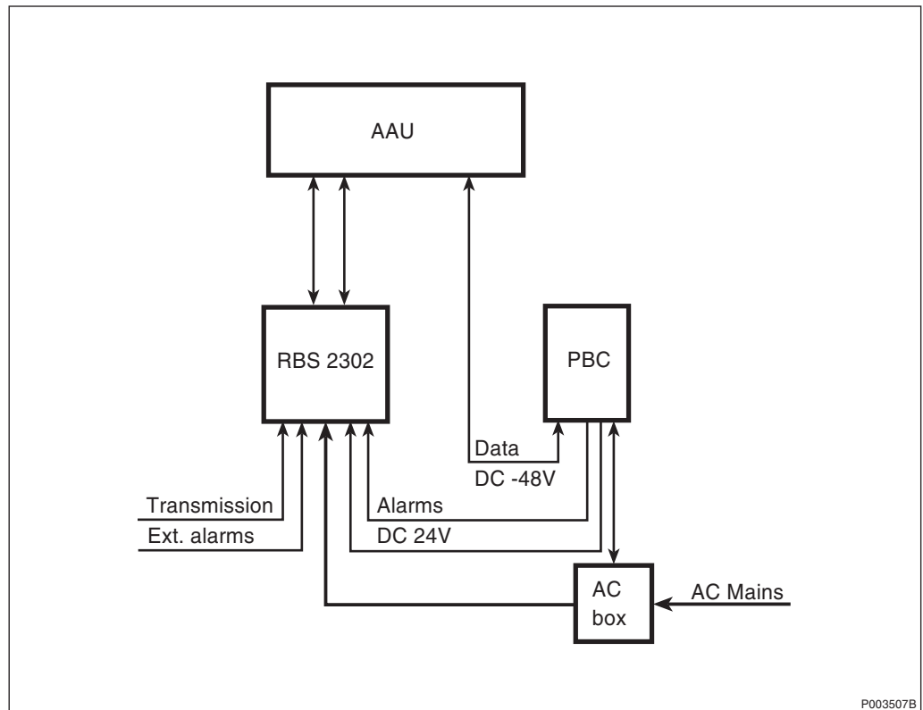
Figure 13 Basic Configuration 2 TRX (R1P1A1)
