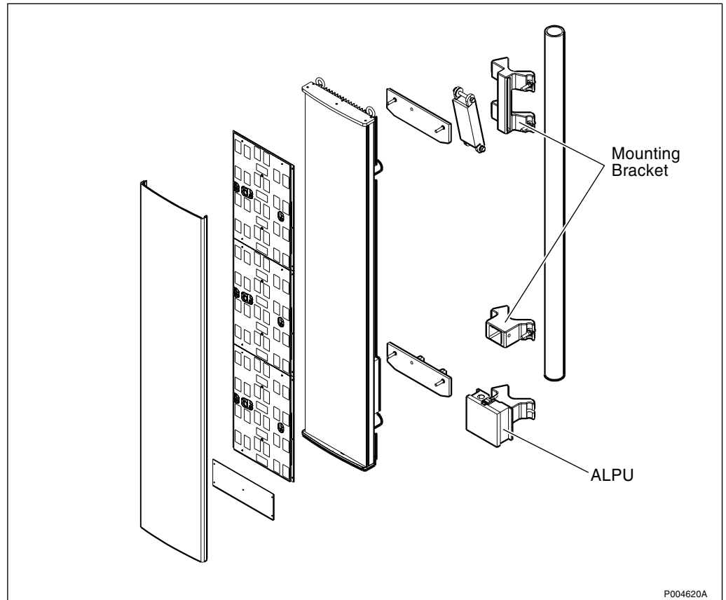
Figure 71 500 W AAU shown with mounting bracket and ALPU
