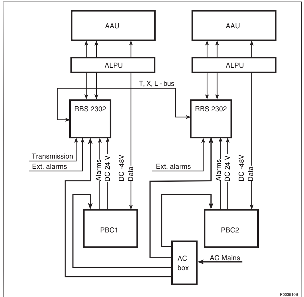
Figure 18 Basic configuration 4 TRX with optional Lightning Protection (R2P2A2AL2)
