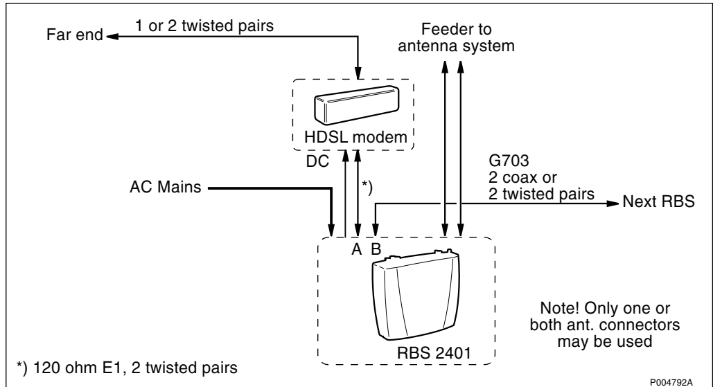
Figure 27 2 TRX with HDSL-modem, HDSL/G.703 (R1H1)
