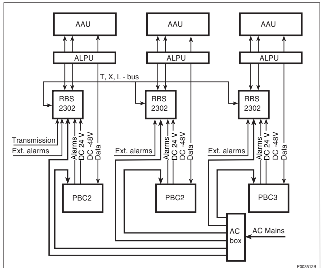
Figure 21 Basic configurations 6 TRX with optional Lightning Protection (R3P3A3AL3)
