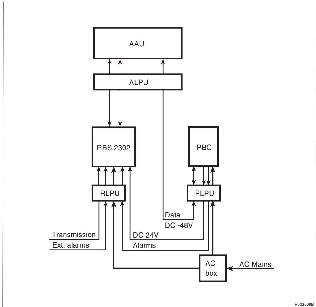
Figure 15 Basic Configuration 2 TRX with optional Lightning Protection (R1P1A1A1)
