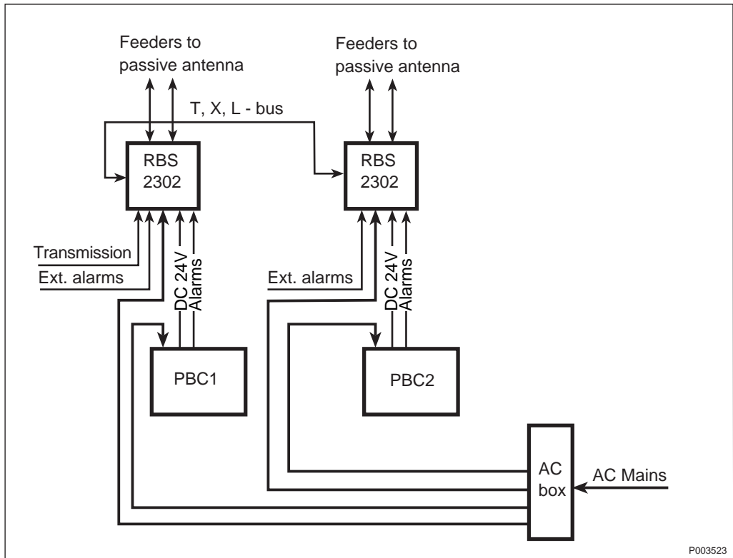
Figure 9 Extended backup, 4 TRX (R2P1)
