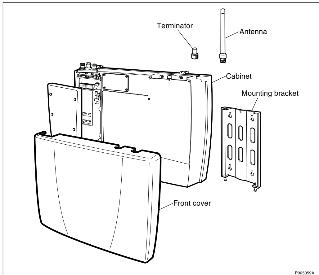
Figure 63 The RBS 2401 cabinet including front cover and mounting bracket seen from different views and the mounting bracket separate
