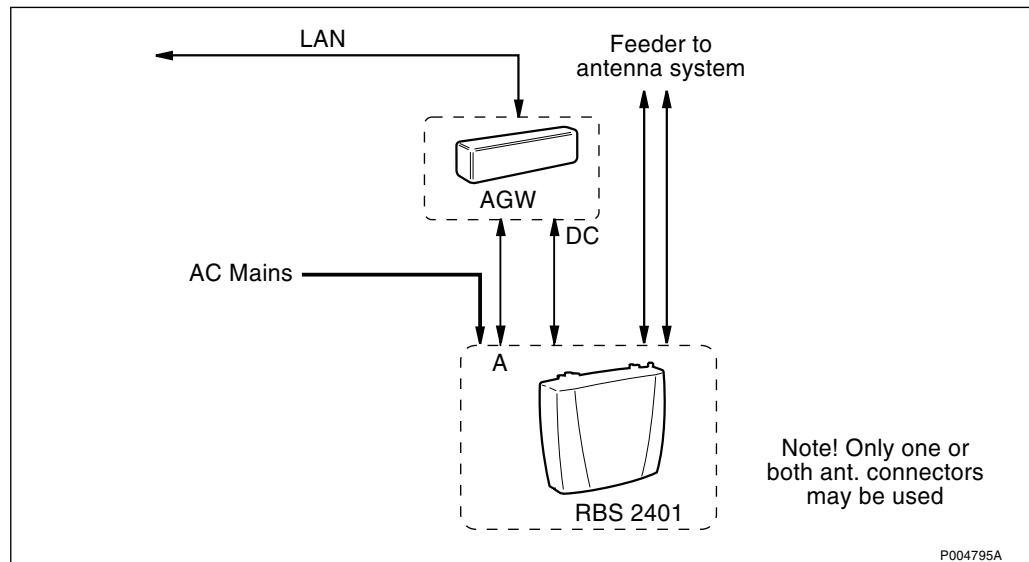
Figure 30 2 TRX, AGW (RIA1)
