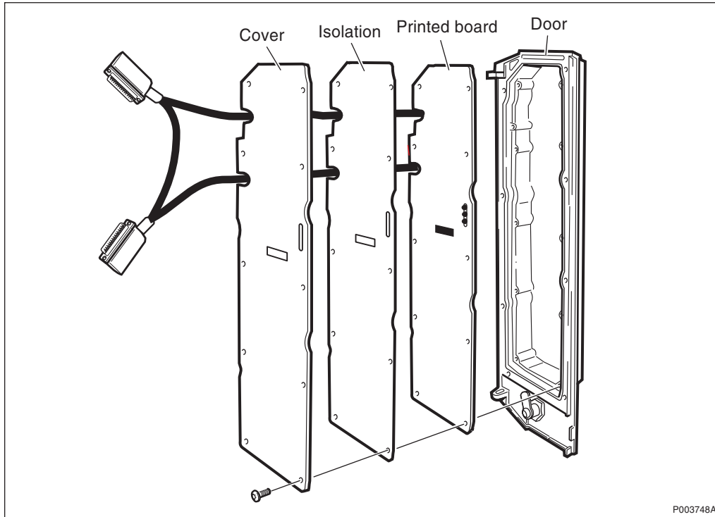
Figure 113 Mounting of HDSL Modem Module in the RBS door
