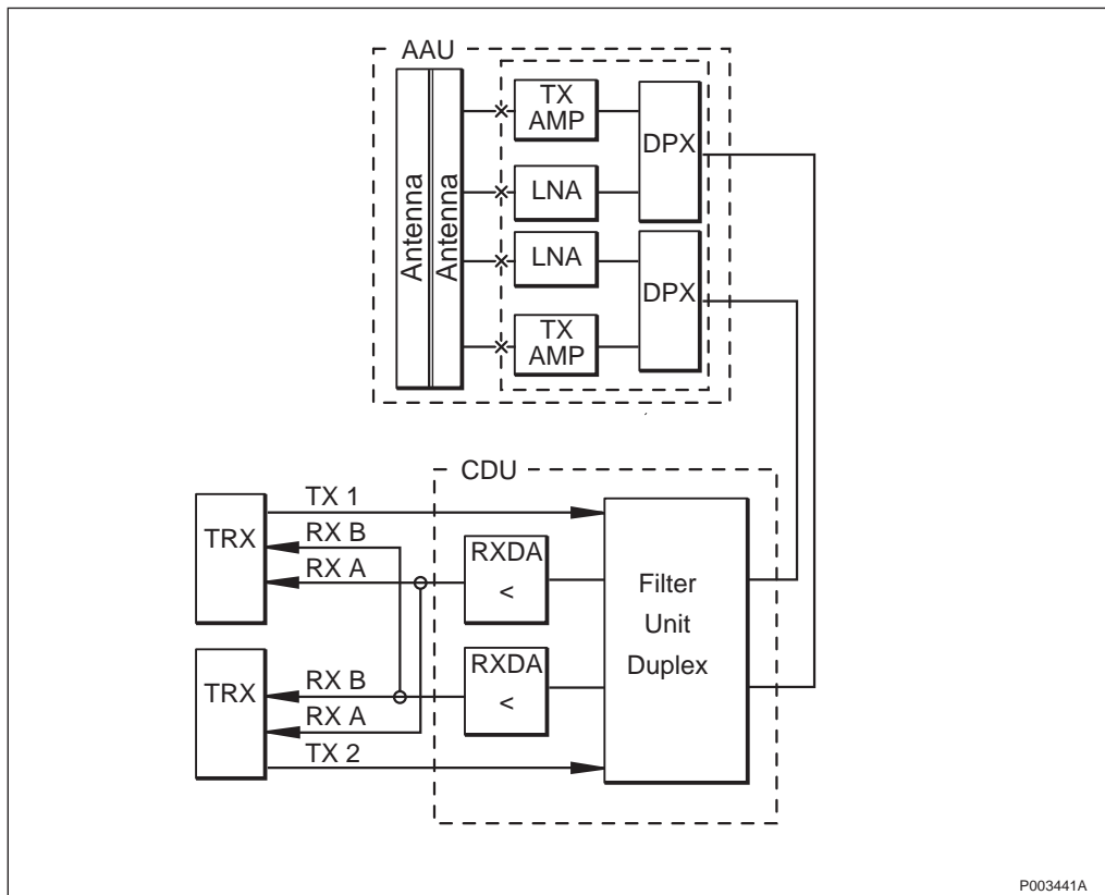
Figure 44 Basic configuration M19d_2.2\A
