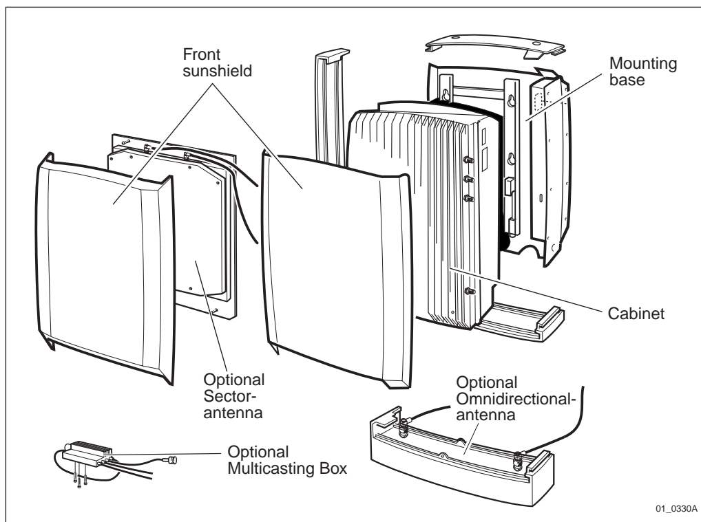
Figure 49 Main physical units
