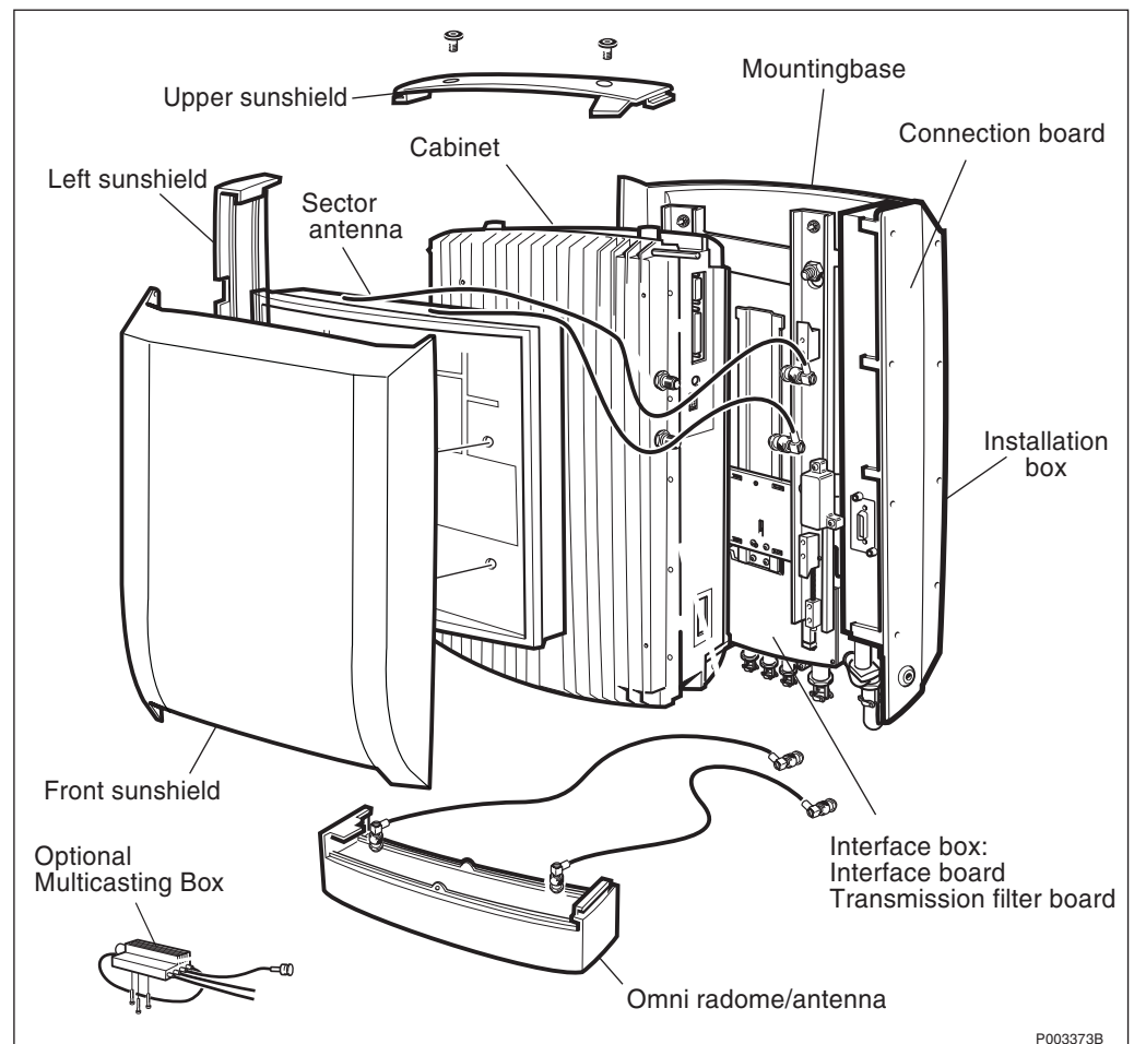
Figure 56 Main Physical Units
