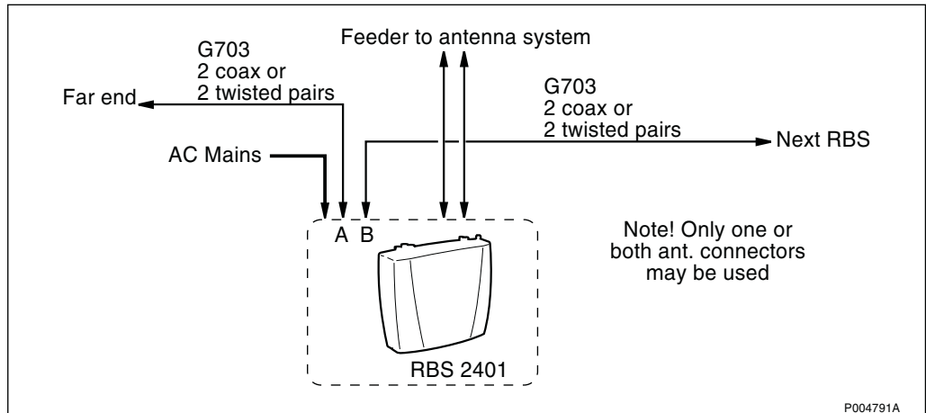
Figure 26 2 TRX (R1)
