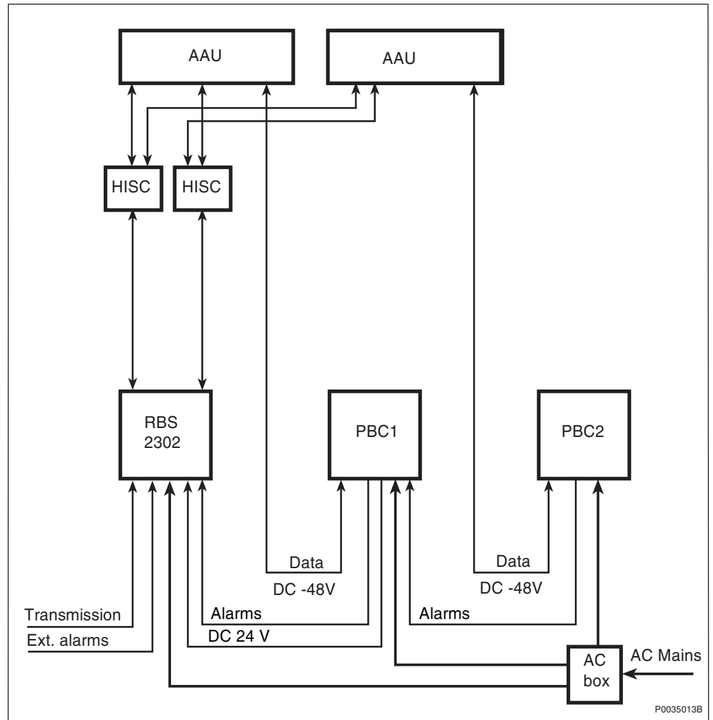
Figure 23 Highway Configuration 2 TRX (RIP2A2H1)
