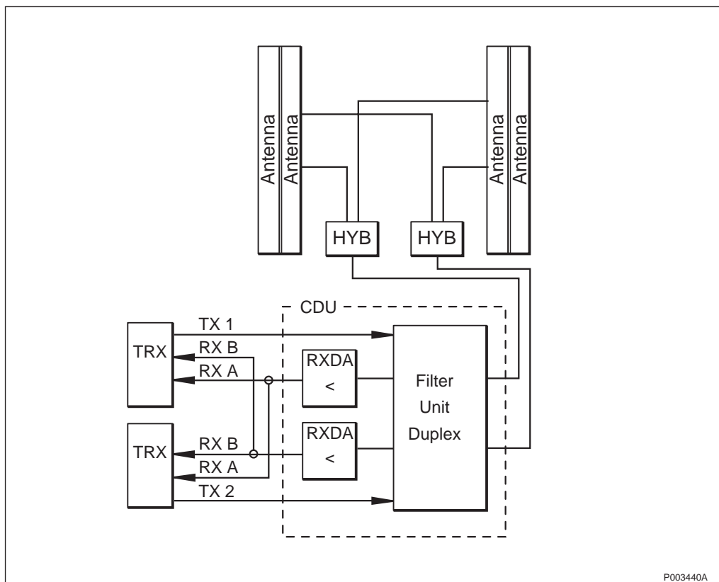
Figure 45 Basic configuration M19d_2.2\H
