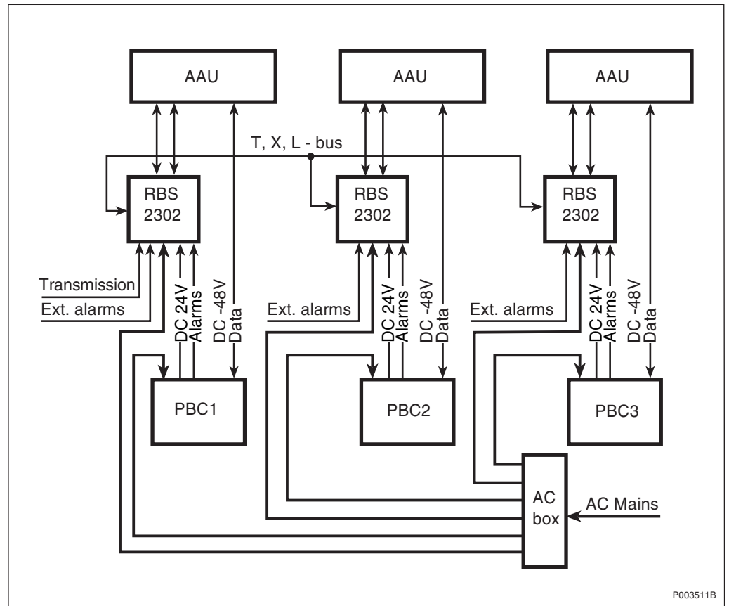
Figure 20 Basic configuration 6 TRX (R3P3A3)
