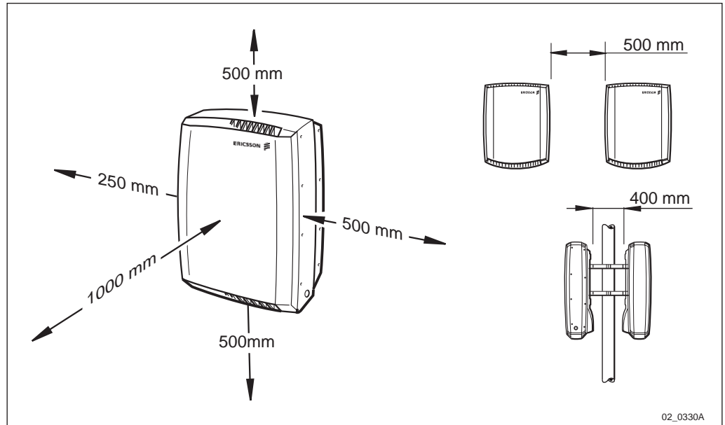
Figure 54 Required separation between RBSs
