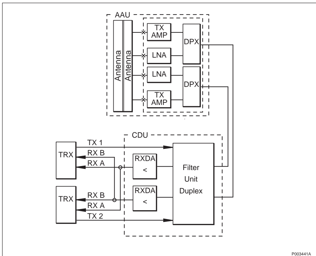
Figure 40 Basic configuration M18d_2.2\A
