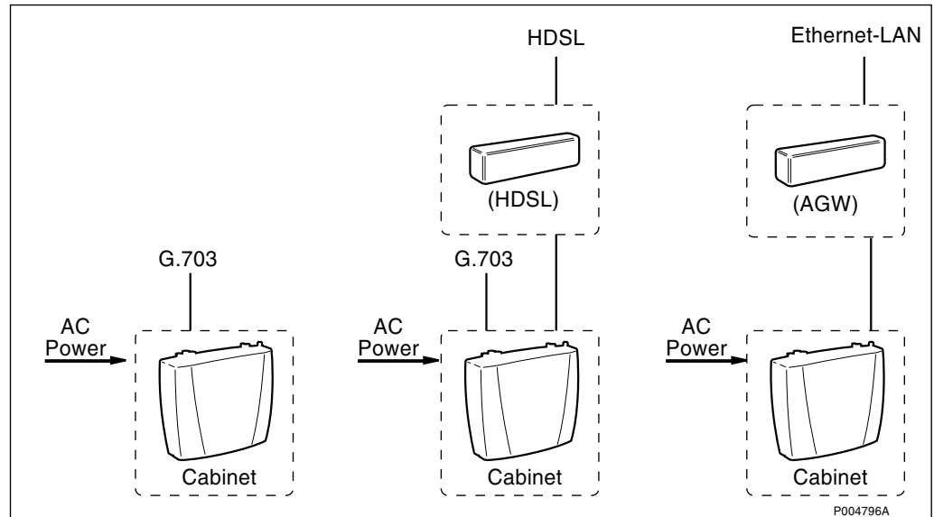
Figure 62 Example of RBS 2401 sites
