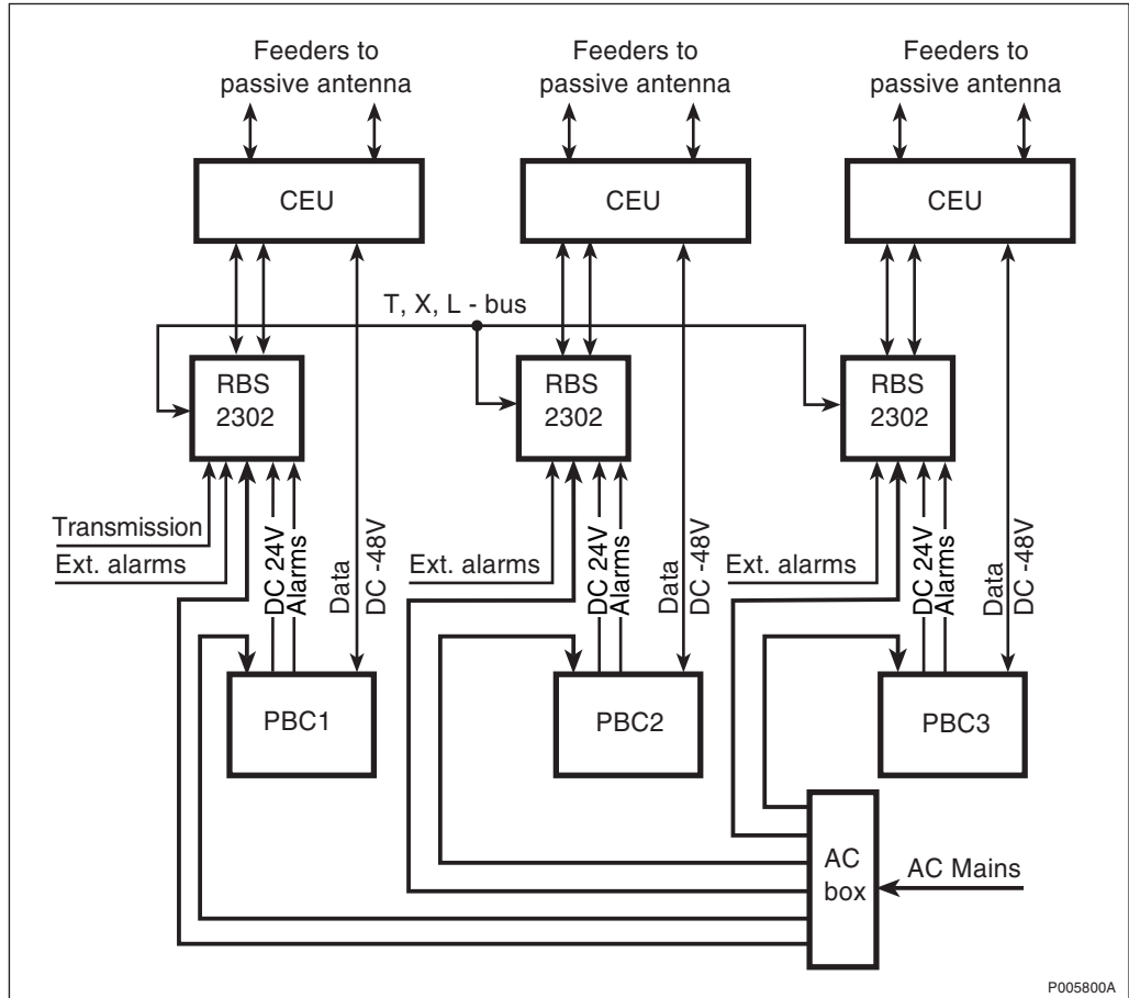
Figure 19 Basic configuration 6 TRX (R3P3A3)
