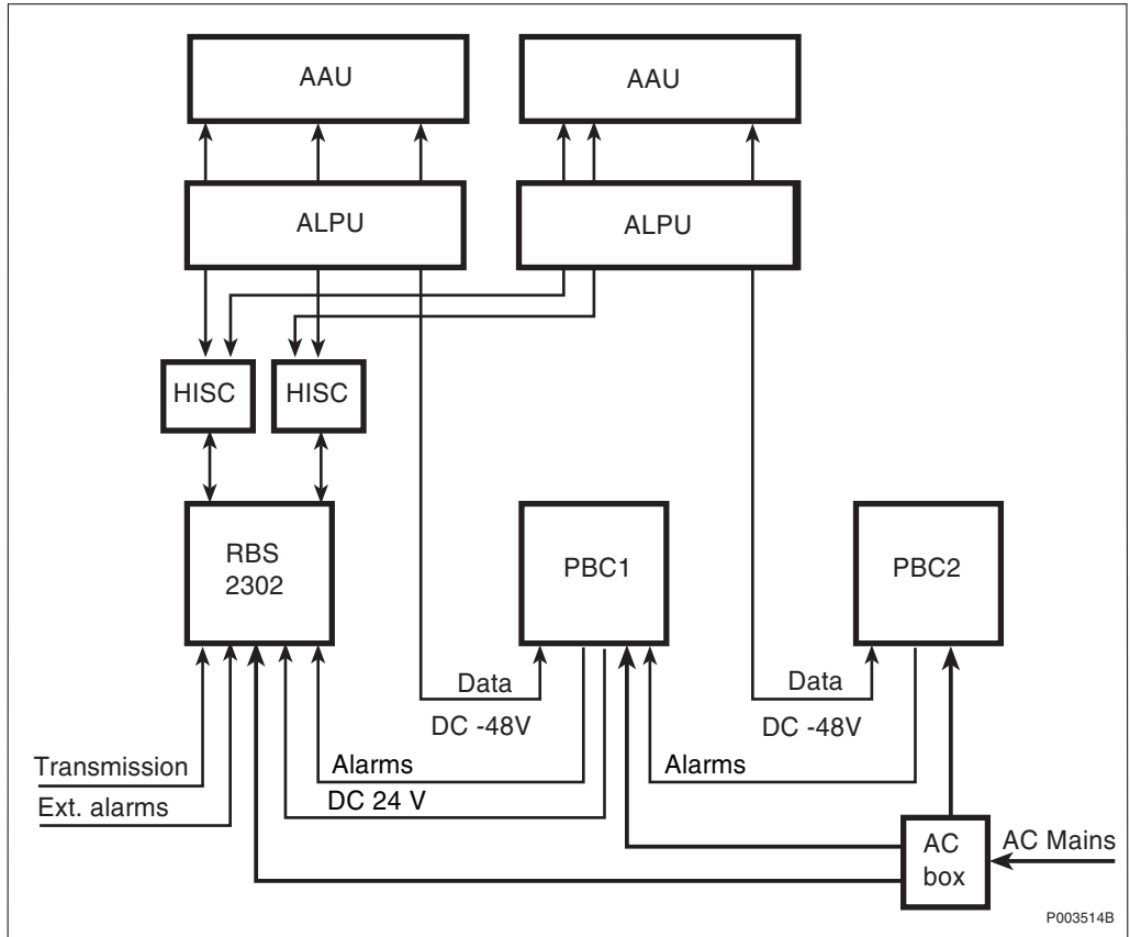
Figure 24 Highway Configuration 2 TRX with optional Lightning Protection (R1P2A2H1AL2)
