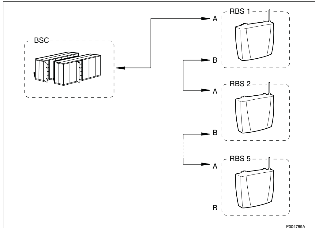
Figure 64 A multidrop chain with five RBSs
