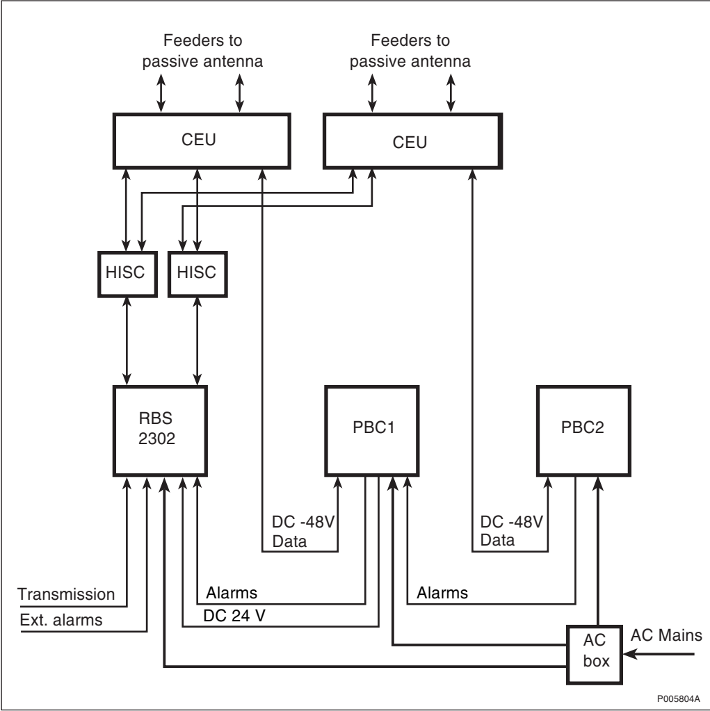
Figure 22 Highway Configuration 2 TRX (R1P2A2H1)
