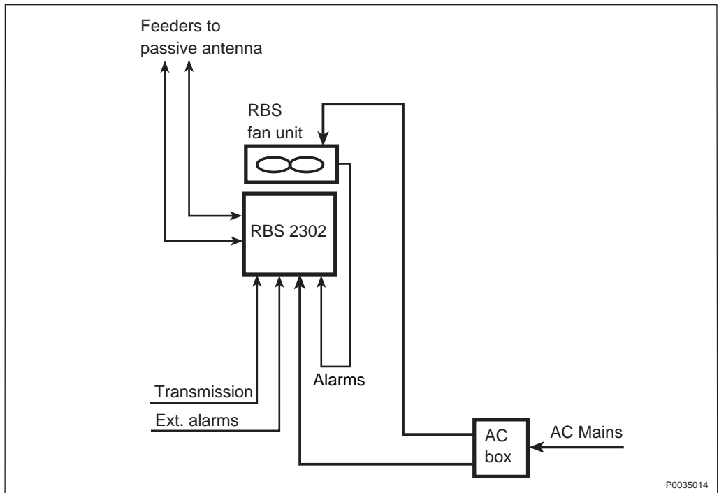
Figure 25 2 TRX, +55°C (R1/RF1)
