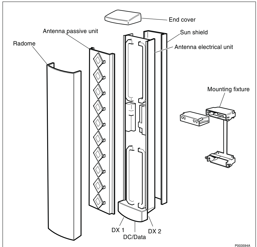
Figure 69 Main physical units, GSM 1800 (500 W)
