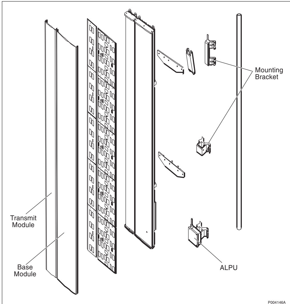
Figure 72 1250 W AAU with mounting bracket and ALPU
