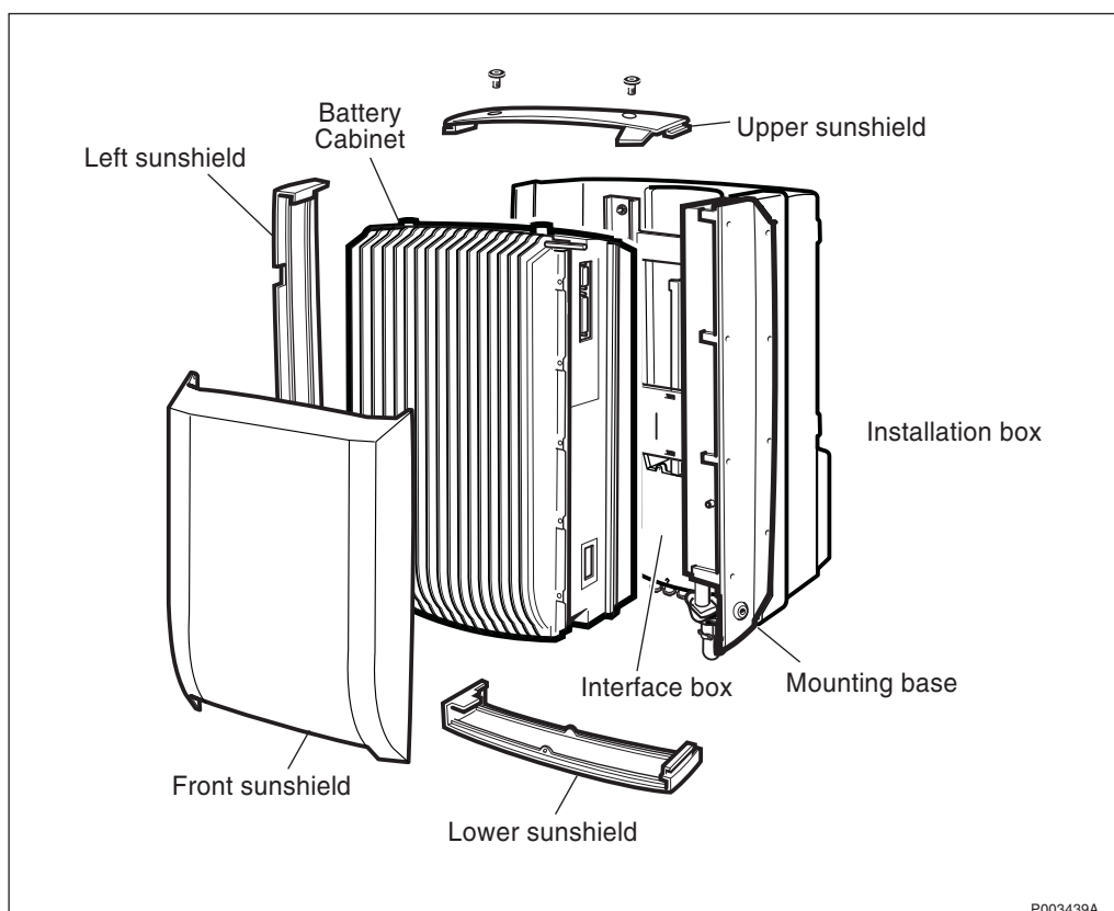
Figure 66 Main Physical Units
