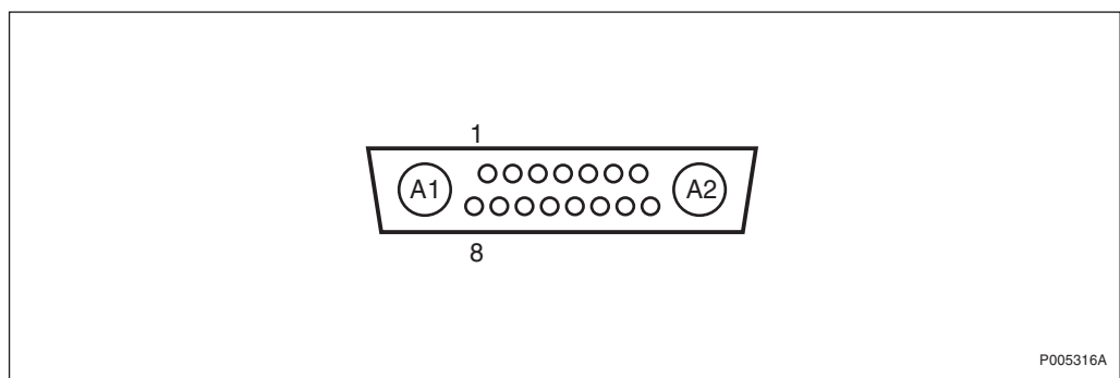
Figure 74 DC/Data connector view from mating side
