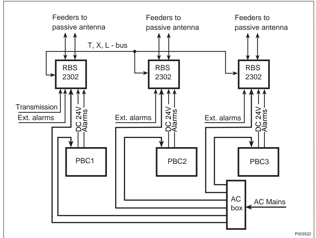
Figure 11 Extended backup, 6 TRX (R3P3)
