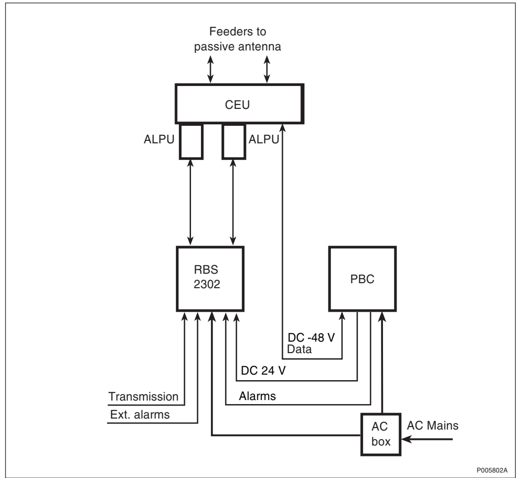
Figure 14 Basic Configuration 2 TRX with optional Lightning Protection (RIP1A1AL1)
