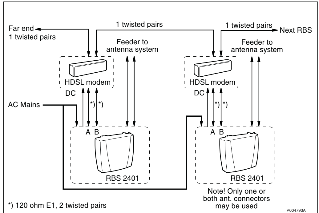
Figure 28 2 TRX with HDSL-modem, HDSL/HDSL (R1H1)
