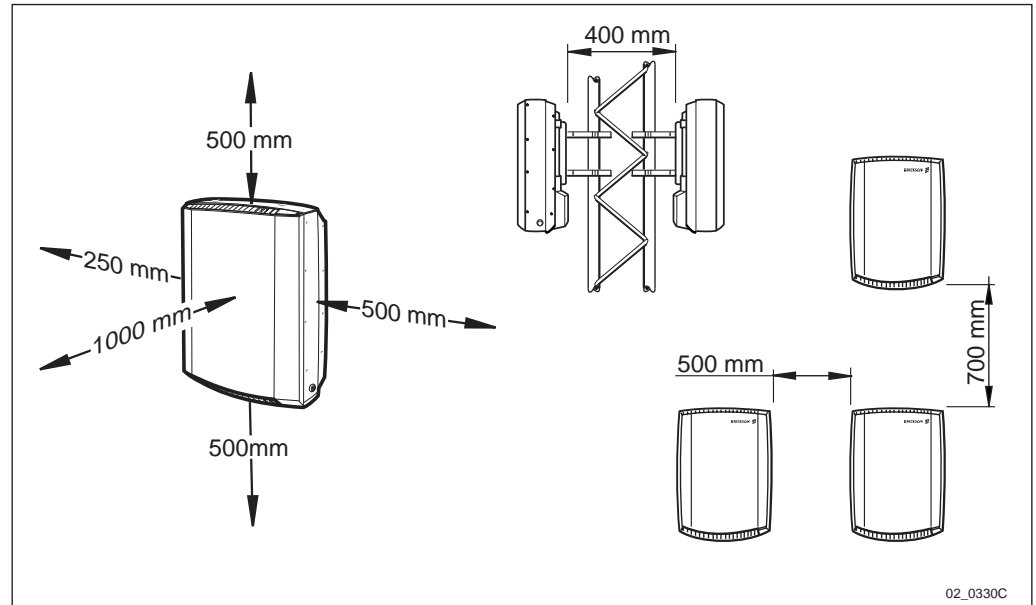
Figure 61 RBS 2302 space requirements
