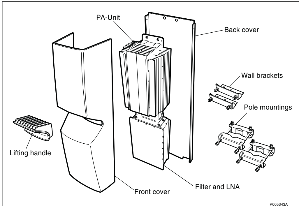
Figure 73 CEU, GSM 900
