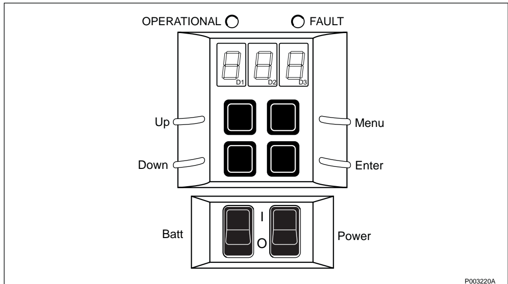
Figure 67 MMI Interface
